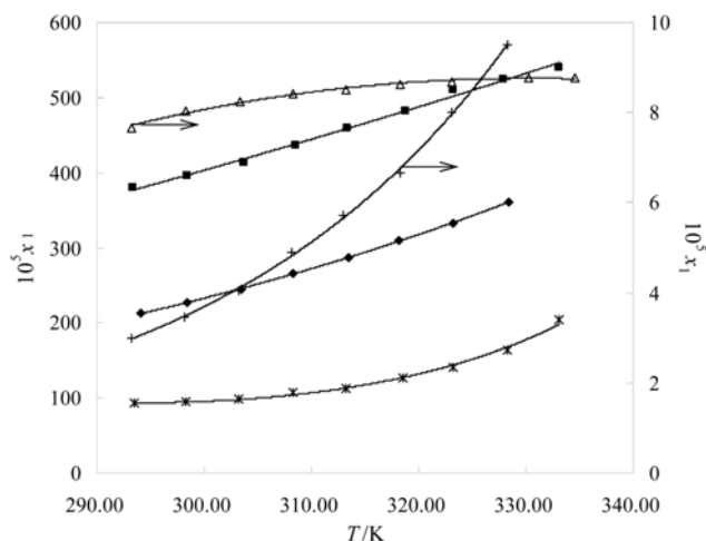
Fig. 2. Mole fraction solubility of L-p -HPG x_1 in different solvent: \blacklozenge , water; \triangle , ethanol; \blacksquare , ethylene glycol; * , dimethyl sulfoxide; + , N,N -dimethylformamide; and solid lines are from calculations by Eq. (2).
